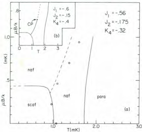
FIG. 1. (a) Phase diagram of ^3\text{He} below 3 mK as determined by experiment of Ref. 7 (open circles) and according to mean-field theory based on coefficients shown. (b) Inset shows how first-order transition with critical point (CP) can be obtained with slight adjustment of parameters.
